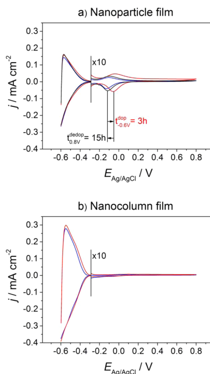
Figure 1. CVs for rutile TiO 2 NP (a) and NC (b) electrodes before and after an electrochemical doping at E_{\text{Ag}/\text{AgCl}} = -0.6 V for 3 h. For the NP electrode the effect of subsequent polarization for 15 h at 0.8 V (dedoping) is also shown. Electrolyte: N 2 -flushed 1 M methanol/0.1 M HClO 4 aqueous solution.
